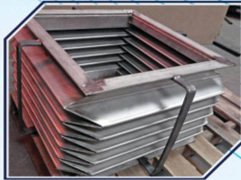
Square Expansion Bellow
