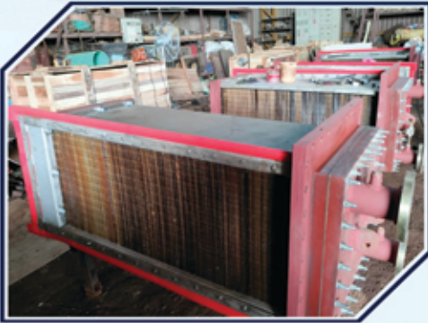
HP & LP Inter Cooler
