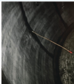
SPARK TEST AFTER RUBBER LINING
