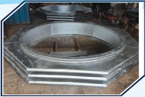
Hexagonal Expansion Bellow
