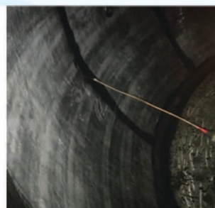
SPARK TEST AFTER RUBBER LINING
