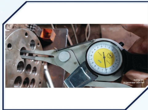
Bore Gauge
